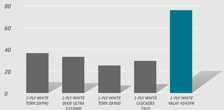
WET STRENGTH (N/m) HIGHER THE NUMBER, HIGHER THE WET STRENGTH
